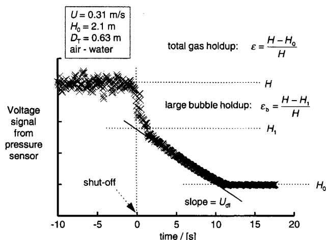
Figure 2. Typical dynamic gas disengagement experiment for 0.63-m-dia. column.
